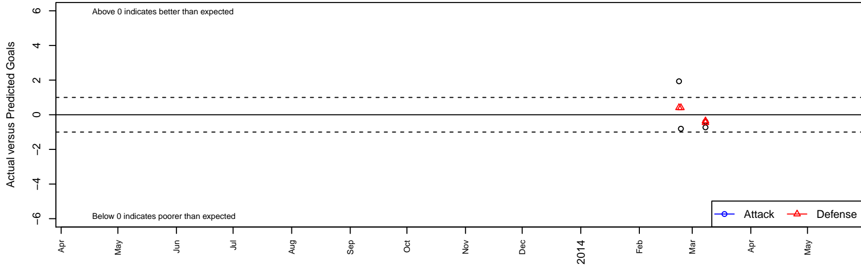
La Esperanza B01 Dots are actual minus expected GF (blue circles) and GA (red triangles). Blue line is smoothed change in attack strength. Red is smoothed change in defense strength.
